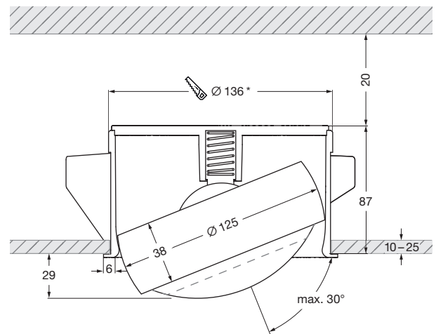
VOLT — Più with lens - - - - Più R with cone glass * cut-out dimensions Installation depth: 107 mm dimensions in mm
